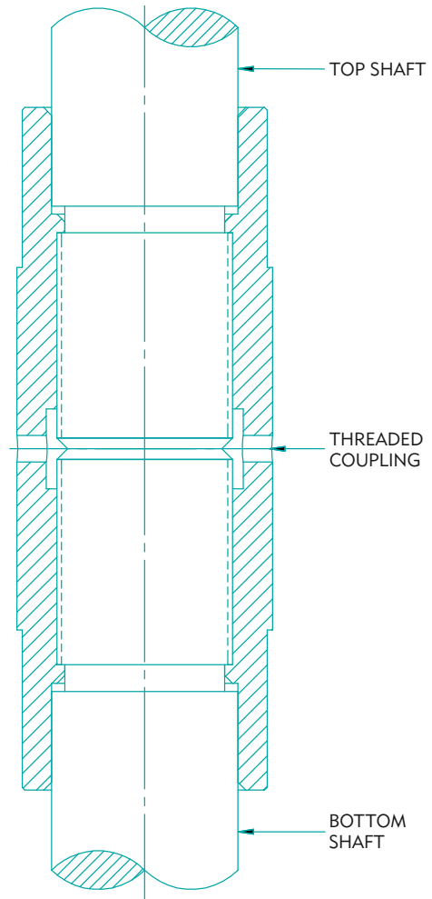
THREADED COUPLING
