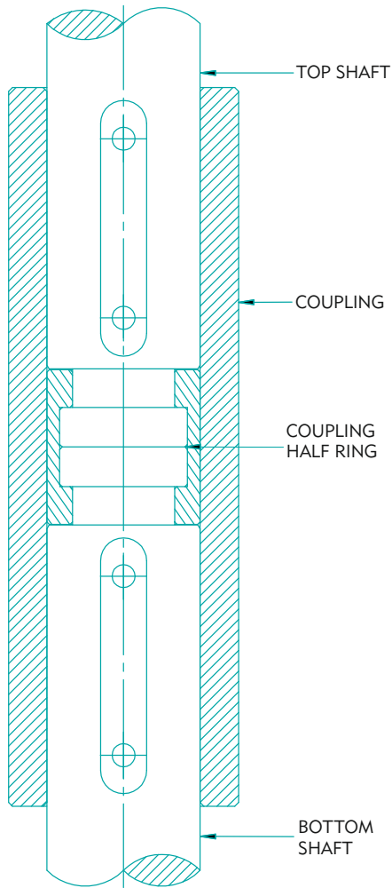
MUFF COUPLING
